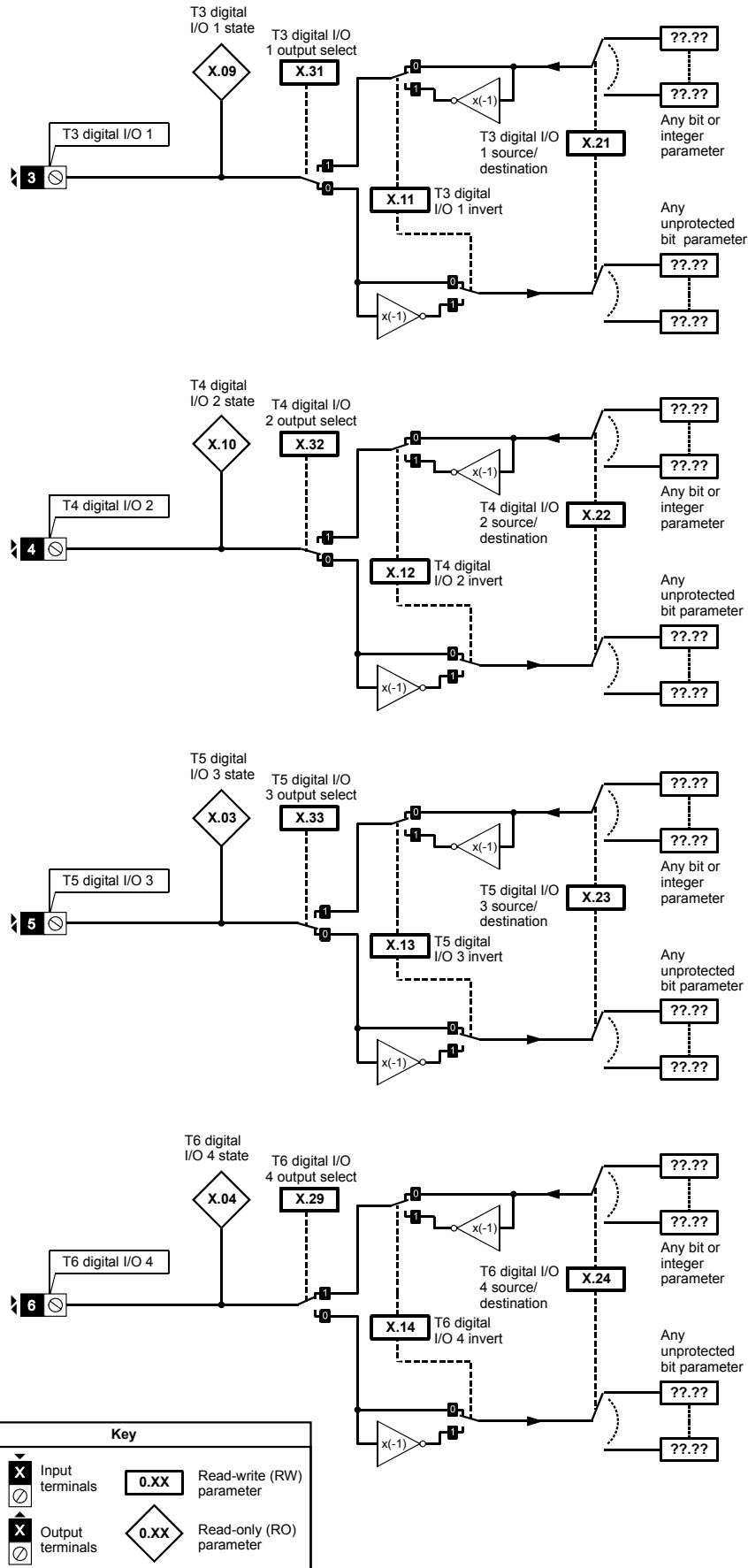
Figure 13-35 SM-I/O PELV digital I/O logic diagram
