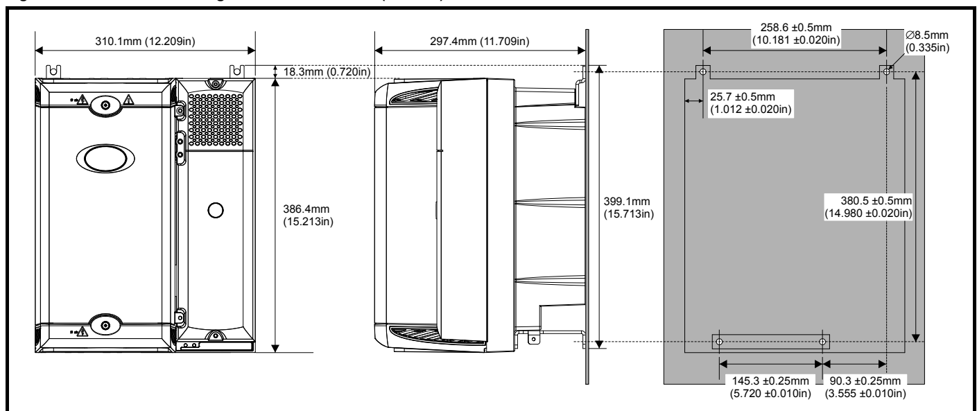
Figure 5-18 Surface mounting the Unidrive SPMC/U (rectifier)
