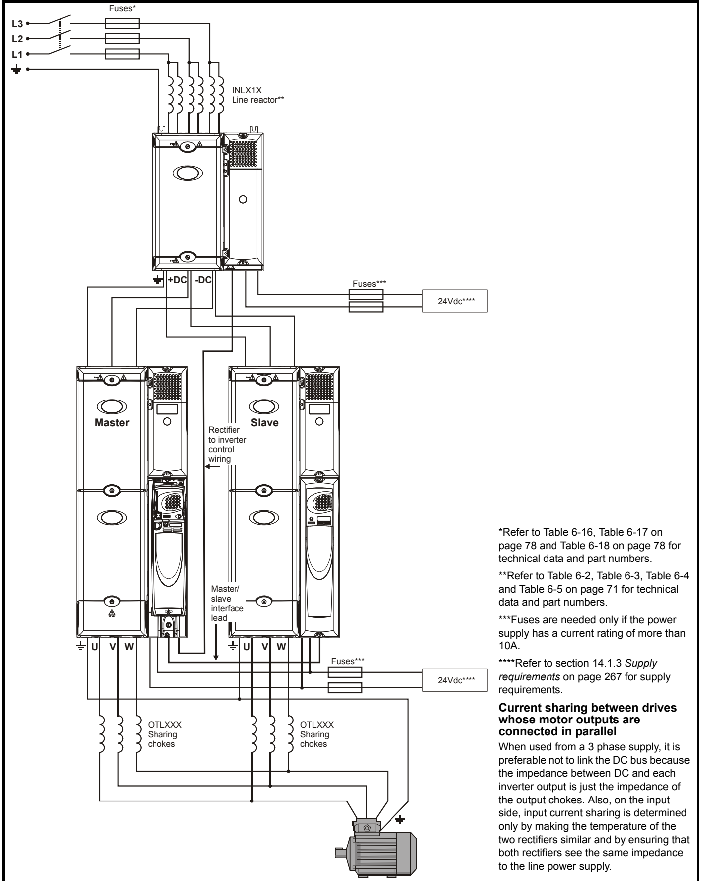
Figure 4-6 Layout for two Unidrive SPMD modules with a dual SPMC rectifier operating on a 3-phase AC supply
