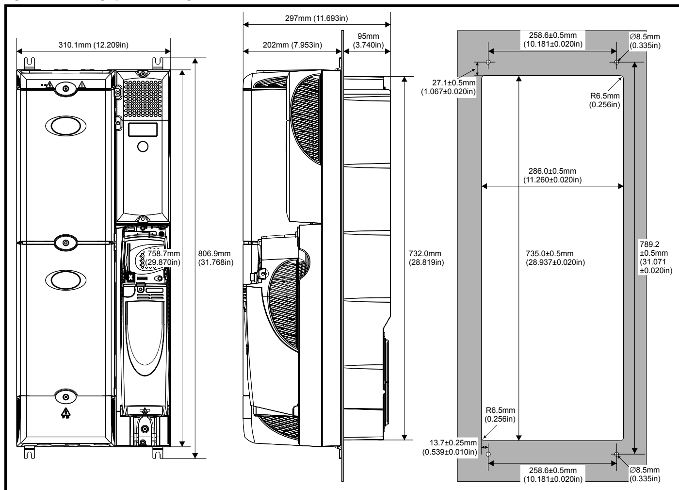
Figure 5-22 Through-panel mounting the Unidrive SPMC/U (rectifier)
