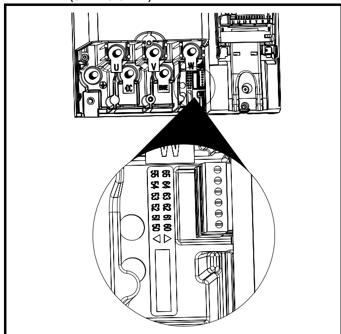
Figure 6-13 Heatsink fan supply connections (SPMA & SPMD)
