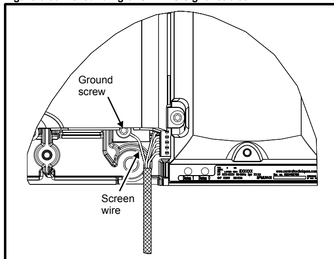
Figure 6-30 Grounding of SPMC/U signal cables
