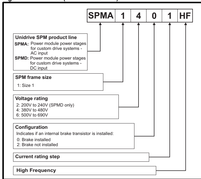
Figure 2-12 Drives (SPMA and SPMD)
