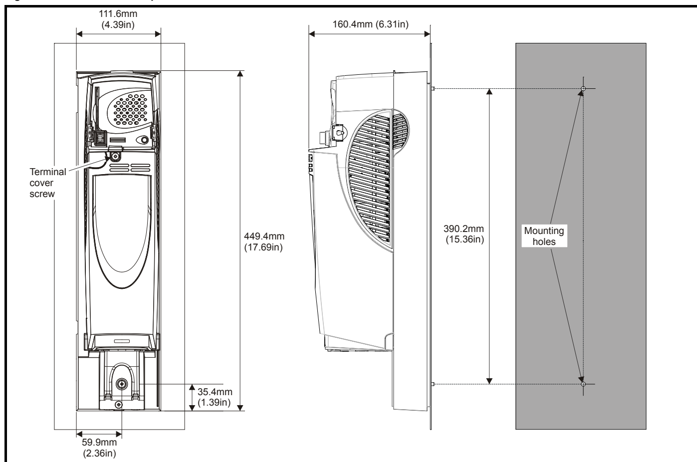
Figure 5-13 Control master pod dimensions
