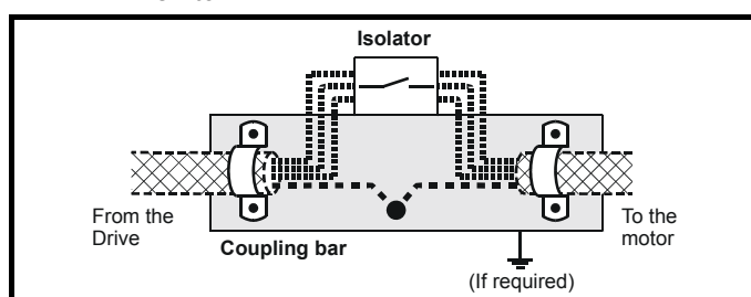
Figure 6-32 Connecting the motor cable to an isolator/disconnect switch
