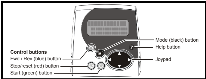
Figure 7-2 SM-Keypad Plus
