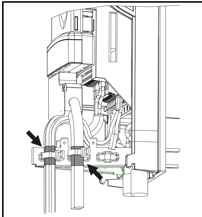
Figure 6-30 Grounding of SPMC/U signal cables
