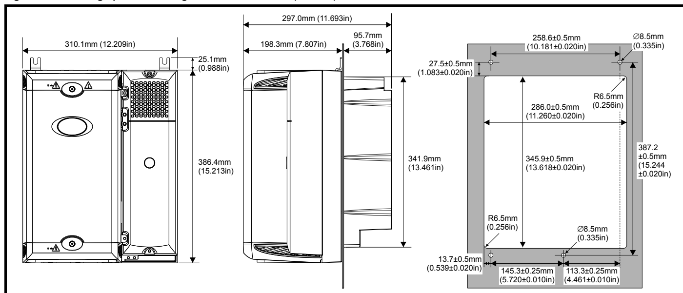
Figure 5-22 Through-panel mounting the Unidrive SPMC/U (rectifier)
