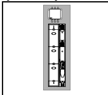
Figure 5-44 Mounting the external EMC filter
